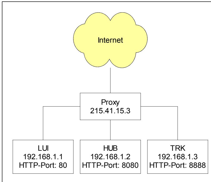
Figure 72 Sample Proxy Setup
