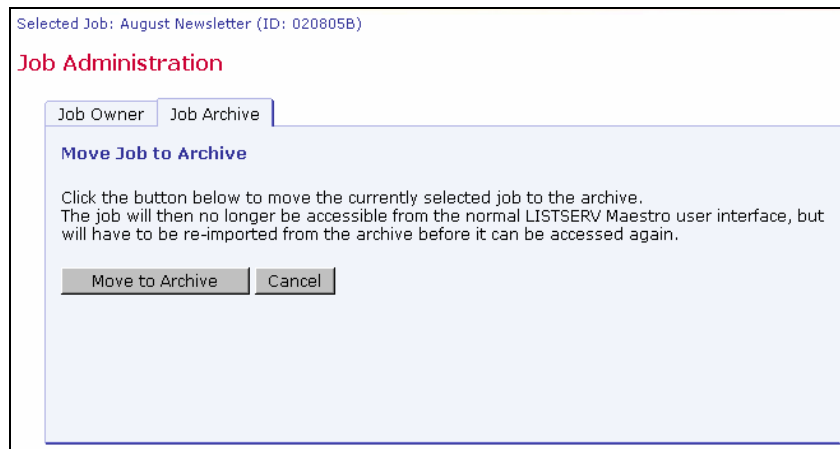
Figure 41 Job Administration - Job Archive
