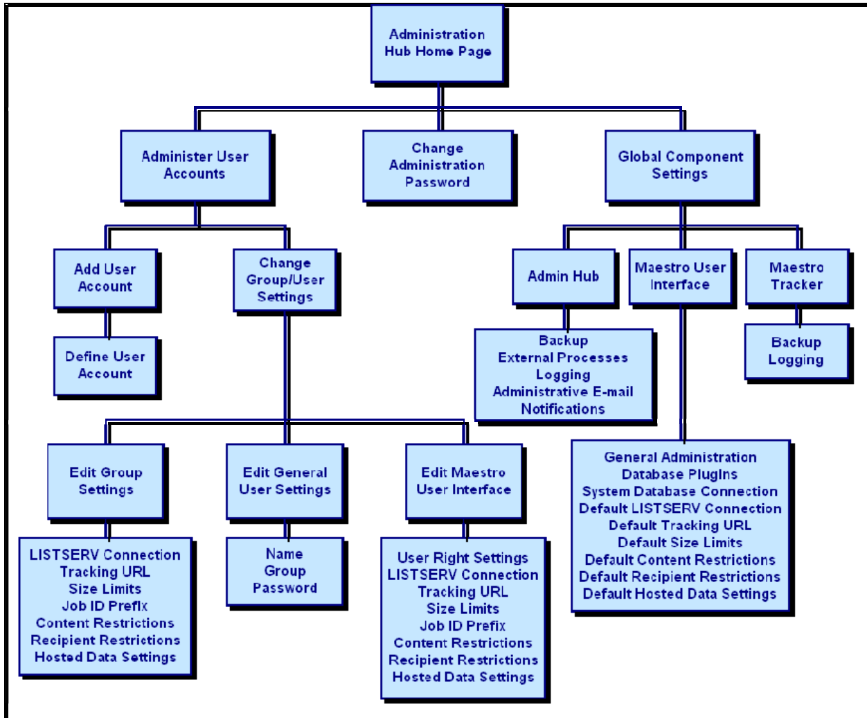
Figure 2 Flow Chart of the Administration Hub
