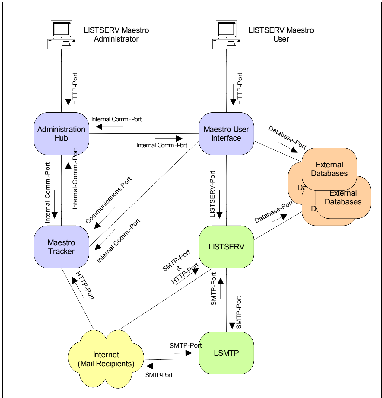
Figure 60 Component Communication Pathways
