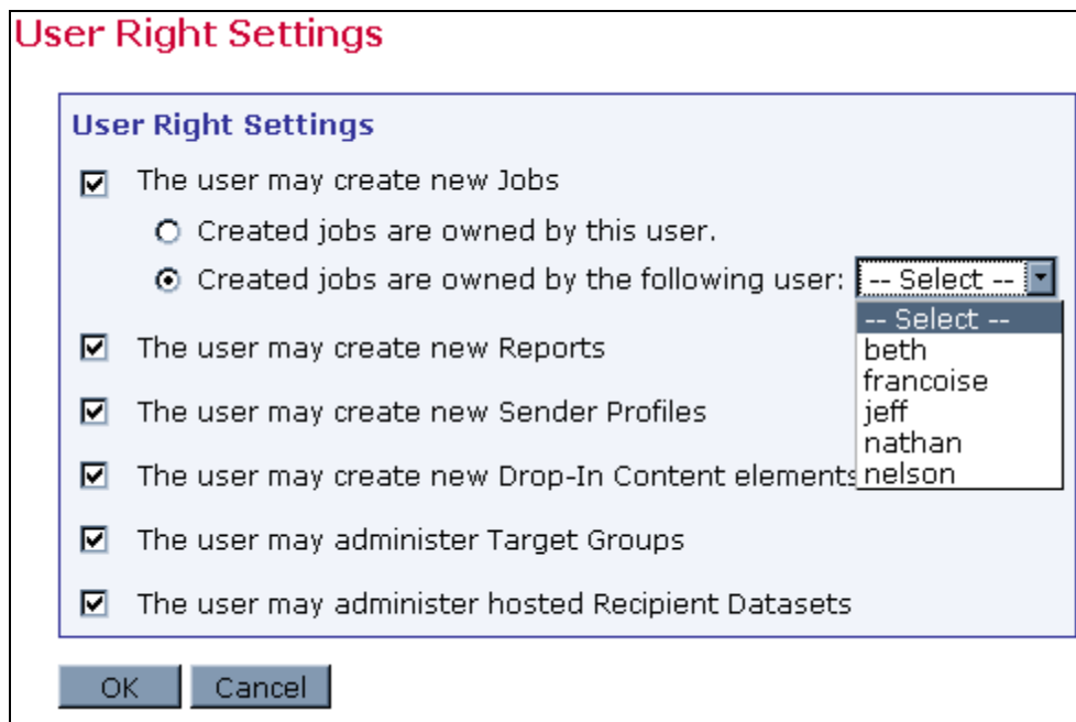
Figure 31 User Right Settings
